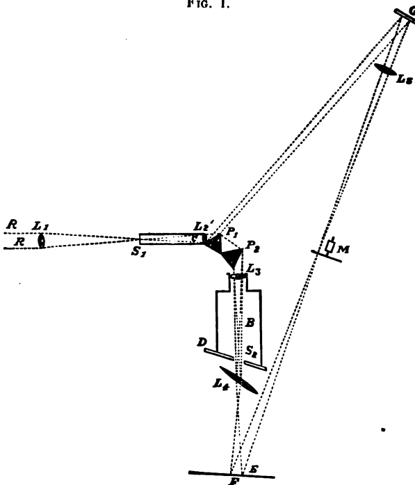
Colour Photometer.
